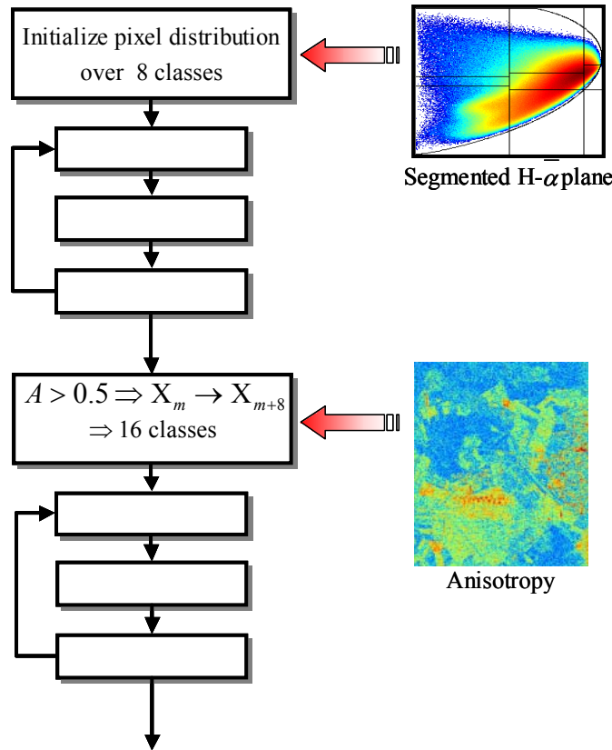
Fig. 11: Synopsis of the Wishart H-A-\alpha segmentation procedure
